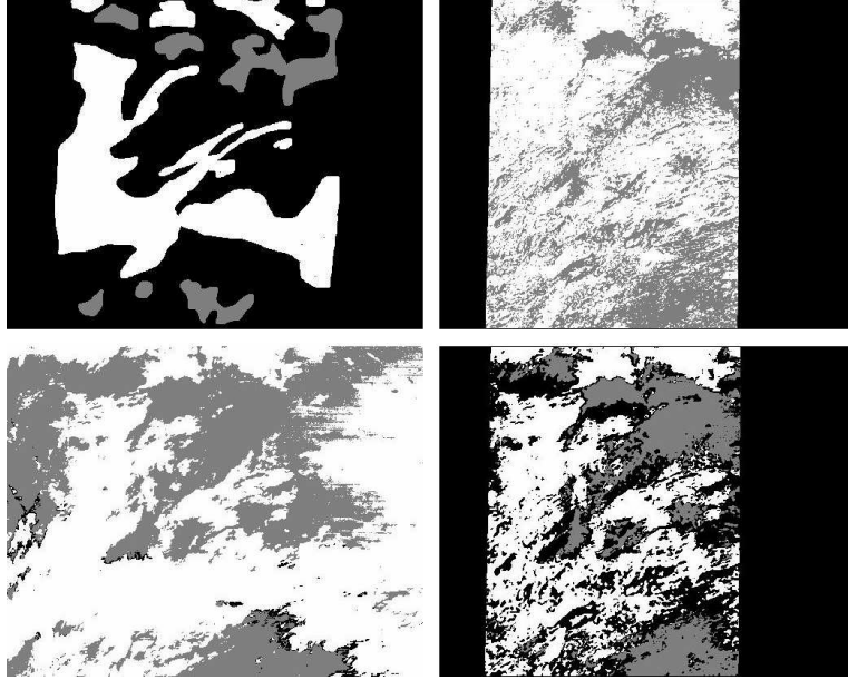
Figure 2: MISR orbit 12558, blocks 25-27. Upper left: expert labels Upper right (white for “cloudy”, gray for “clear” and black for “not sure”): MISR ELCMC result; Lower left: MODIS results; Lower right: Consensus pixels. Coding scheme: white for “cloudy”, gray for “clear”, and black for “no retrieval” or “dis-agree”.
