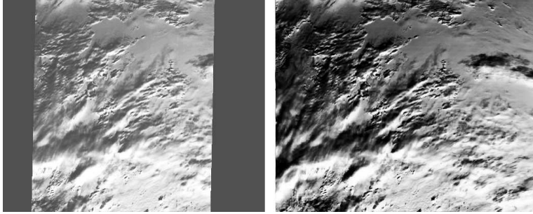
Figure 1: Left: MISR An red image; Right: MODIS band 1 image mapped to MISR grid. MISR orbit 12558, blocks 25-27.
