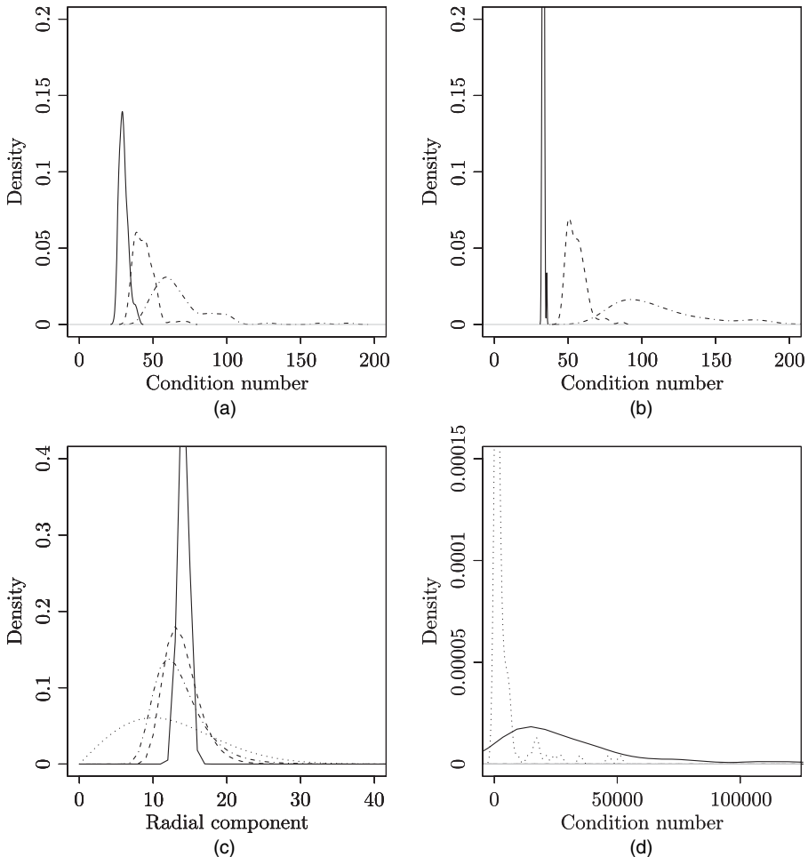
Fig. 10. (a), (b) Estimated densities of the condition number of \bar{p}^{-1}\tilde{\mathbf{Z}}\tilde{\mathbf{Z}}^T , based on 100 simulations, when \mathbf{Y} is Gaussian (—) and multivariate t with \nu = 20 (-----) and \nu = 10 (· · · · ·) degrees of freedom ((a) n = 100 , \bar{p} = 200 ; (b) n = 1000 , \bar{p} = 2000 ), (c) corresponding densities of the radial components of these spherically symmetric densities when \bar{p} = 200 , as well as the density of a scaled Weibull distribution with shape parameter 2 (· · · · ·), and (d) estimated condition number density of \bar{p}^{-1}\mathbf{Z}\mathbf{Z}^T in the Weibull case, with n = 100 , \bar{p} = 200 (· · · · ·) and n = 1000 , \bar{p} = 2000 (—)
