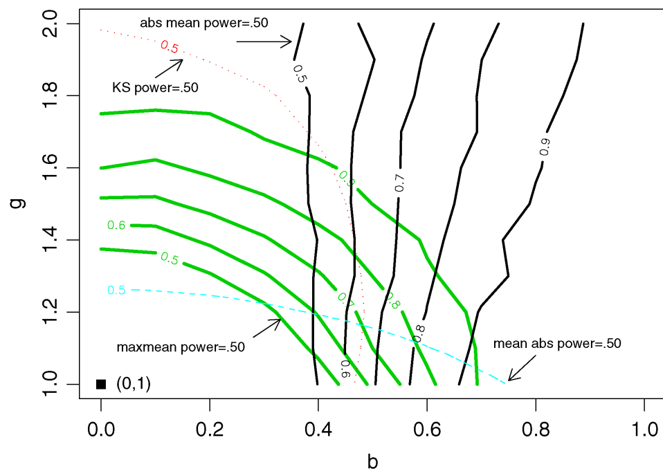
FIG. 5. Contours of equal power for absolute mean, enrichment statistic |\bar{z}_{\mathcal{S}}| (jagged vertical line) mean of absolute value (curving broken line), and maxmean statistic (heavy curving lines); for testing H_0 : z_i \stackrel{\text{ind}}{\sim} N(0, 1) vs N(b, g^2) , i = 1, 2, \dots, m = 25 , at level 0.95; “ks” is 0.5 power contour for the Kolmogorov–Smirnov test, dominated by maxmean test with 0.5 contour everywhere closer to null point (0, 1) . Using mean absolute value, average over \mathcal{S} of |z| has very little power versus shift alternatives, curved dashed line.
