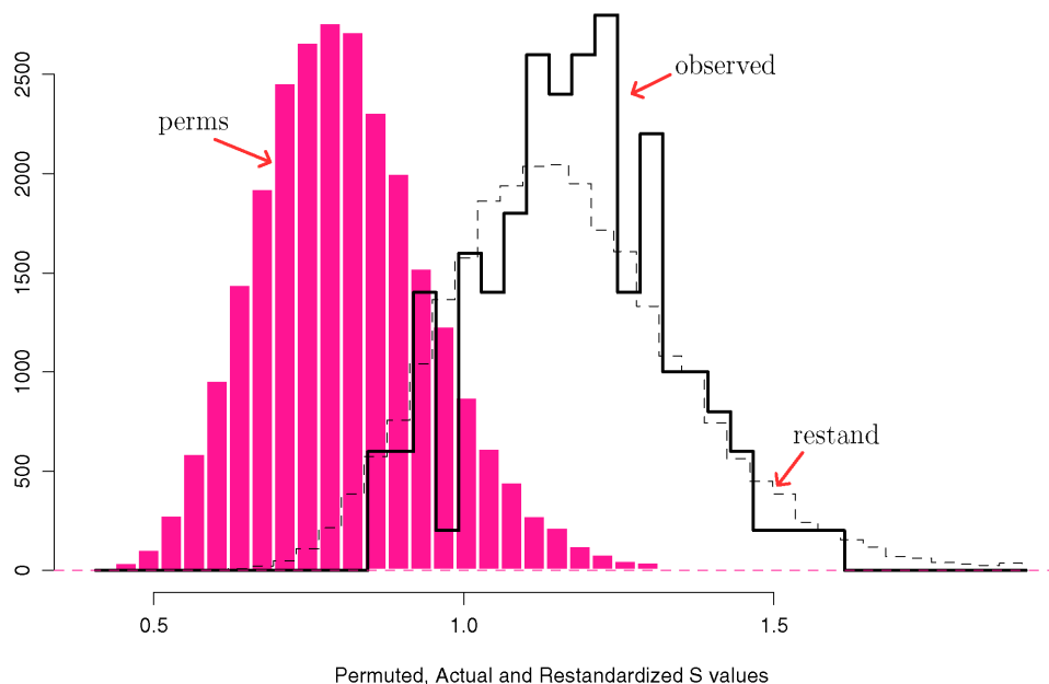
FIG. 4. Enrichment statistics S for 129 randomly selected gene-sets of size m = 25 , heavy line histogram, lies far to right of permutation S^* values, solid histogram. S = \sum_g |z_i|/m , BRCA data, Hedenfalk et al. (2001). Restandardized values (2.12), light line histogram, gives a much better match to actual values.
