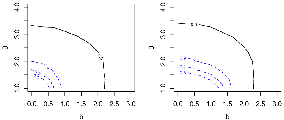
FIG. 6. Contours of power 0.5 (solid lines) for individual gene scores z_i and power 0.5, 0.7...0.9 (broken lines) for the maxmean statistic; for testing H_0: z_i \stackrel{\text{ind}}{\sim} N(0, 1) vs N(\pm b, g^2) , i = 1, 2, \dots, m = 25 . In the left panel, all genes in the gene-set are shifted by b ; in the right panel, half of the genes are shifted by b and half by -b .
