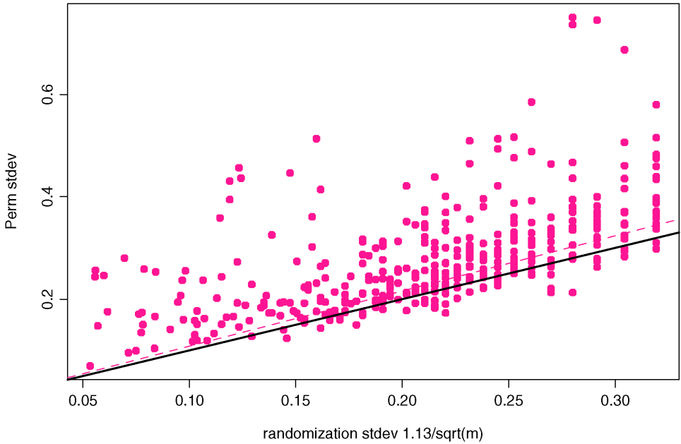
FIG. 3. Permutation standard deviation compared to randomization standard deviation for S = \bar{z}_g , 395 gene-sets for p53 data, Subramanian et al. (2005). Permutation values exceed randomization values, especially for gene-sets with large m at left, reflecting positive correlations within gene-sets.
