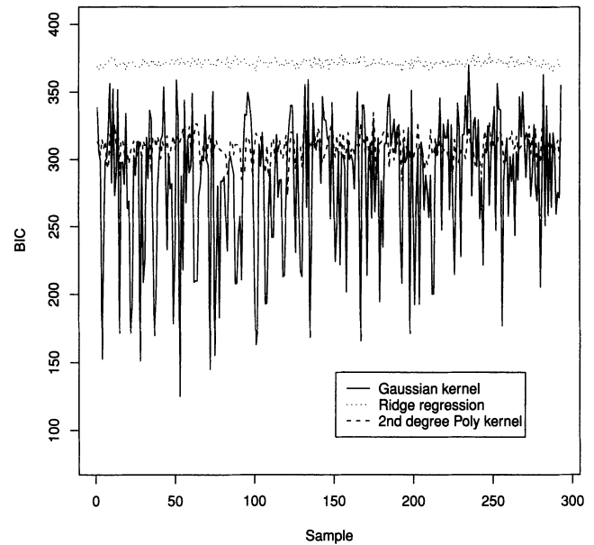
Figure 2. Simulation result of model selection using KM_{BIC} .
